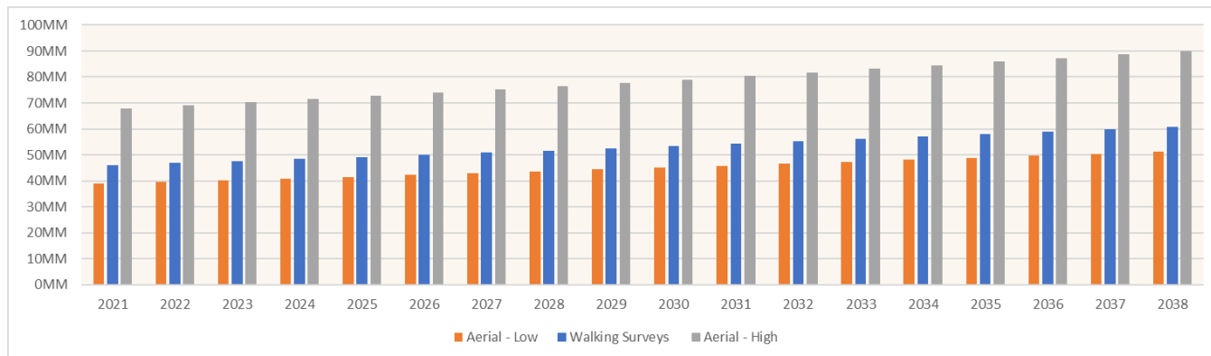
Figure 13. Annual costs for multiple programs considering infrastructure variation. Cost per year includes leak survey cost, follow-up (when applicable) and repair. Cost per mile, per follow-up and per repair reflects the operator's feedback described in section 2.2.3.
