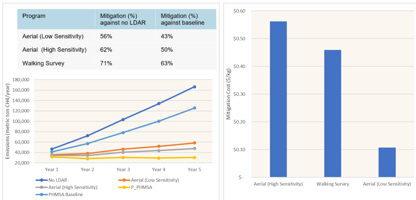
Figure 7. Left side, modelled emissions per year when considering Distribution 1. Right side, mitigation cost ($/ kg of CH 4 avoided - calculated considering cumulative 5-year cost and cumulative 5-year mitigation).
