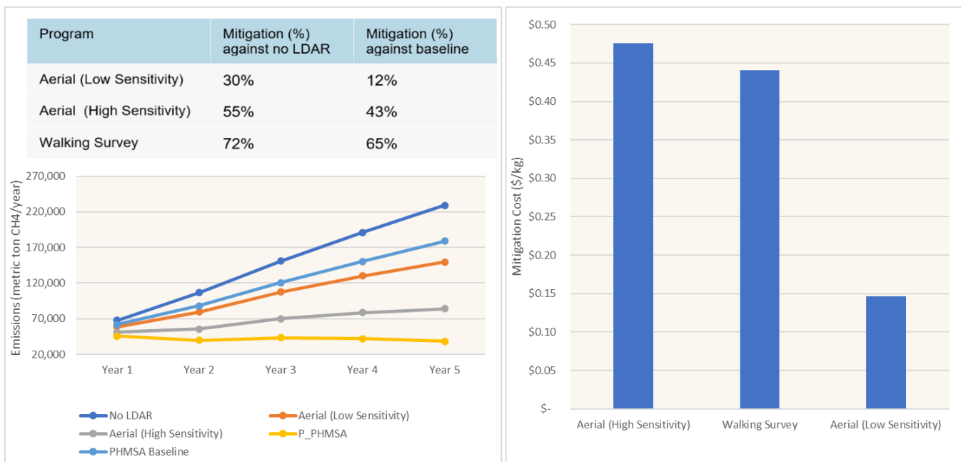
Figure 11. Left side, modelled emissions per year when considering Distribution 2. Right side, mitigation cost ( $/ kg of CH 4 avoided - calculated considering cumulative 5-year cost and cumulative 5-year mitigation)
