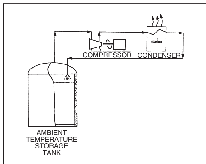
FIG. 6-22 Ambient Temperature Vapor Recovery Cycle
