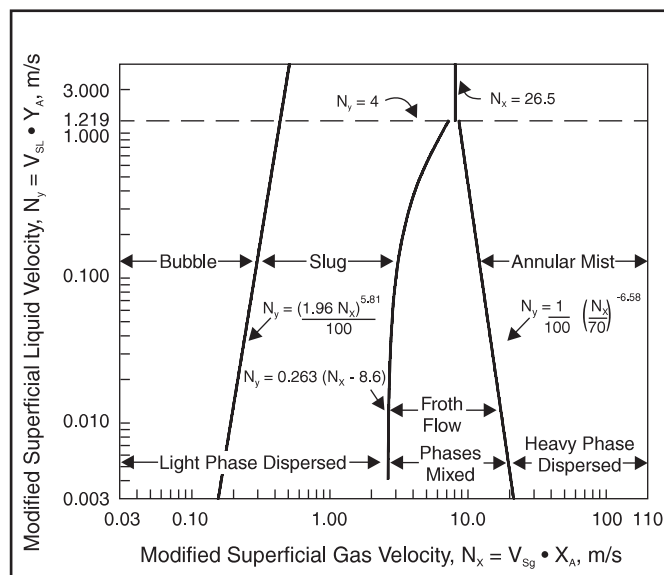
FIG. 17-16 Vertical Up-Flow Regime Map 14
