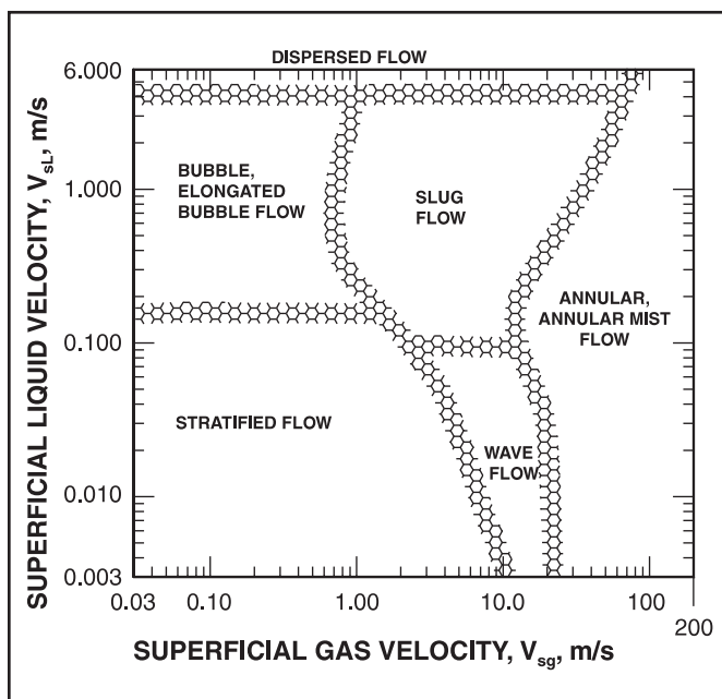
FIG. 17-15 Horizontal Flow Regime Map 12
