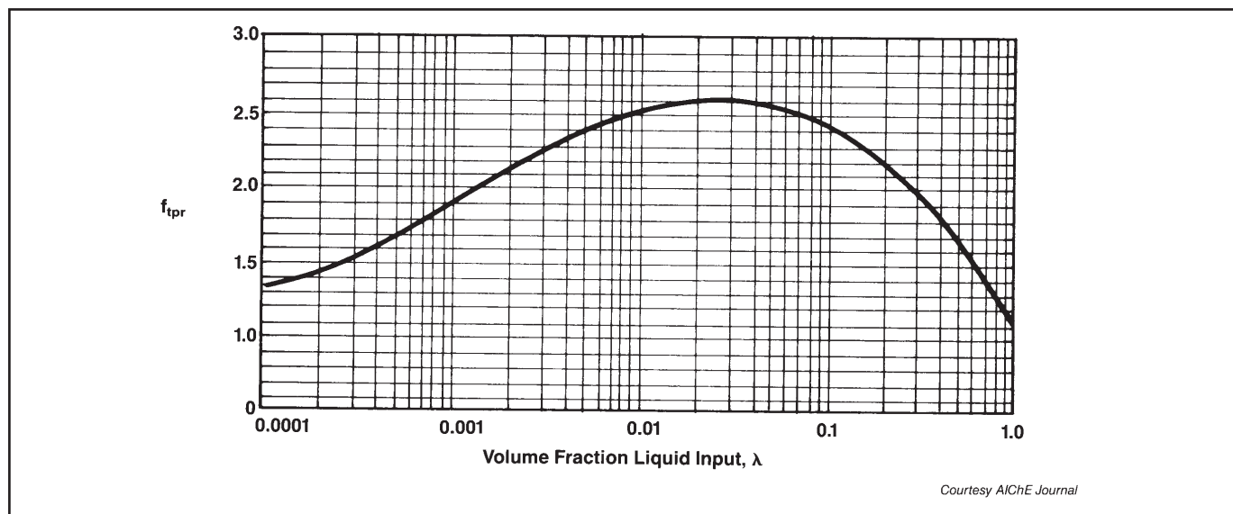
FIG. 17-17 Two-Phase Friction Factor Ratio 18
