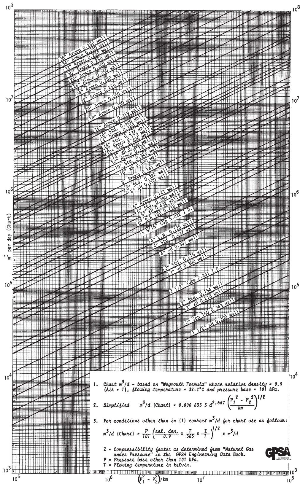
FIG. 17-6b Gas Flow Based on Weymouth Formula
