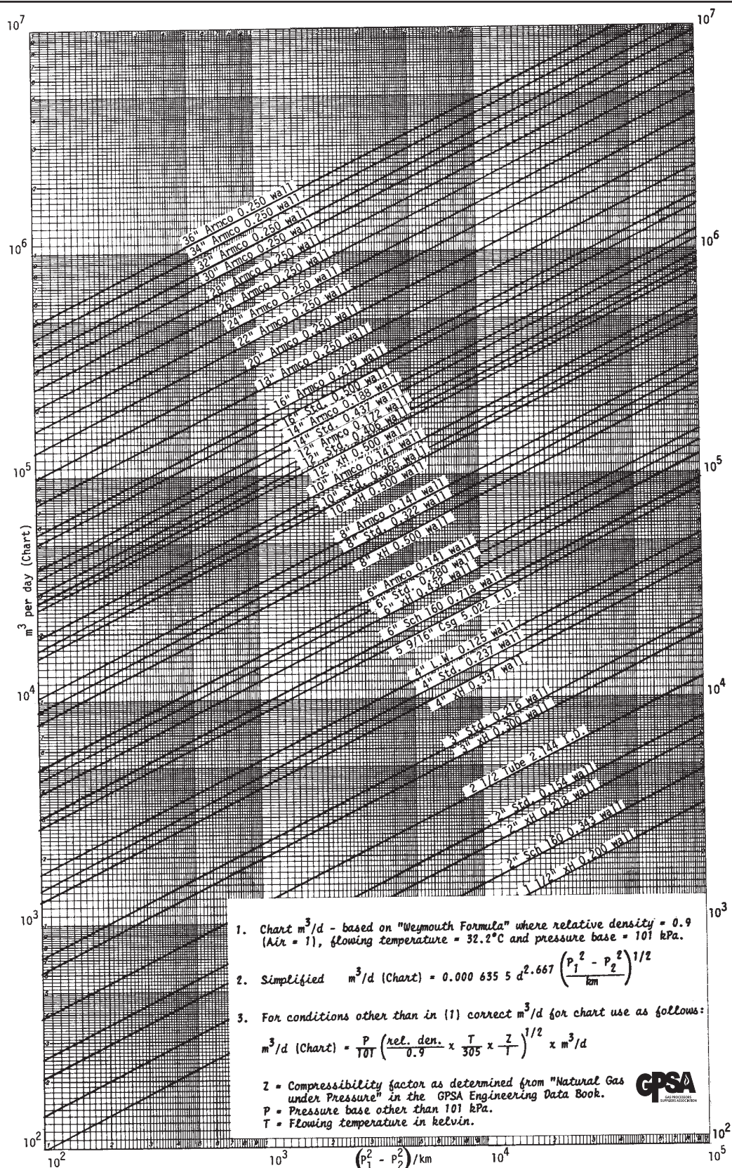
FIG. 17-6a Gas Flow Based on Weymouth Formula
